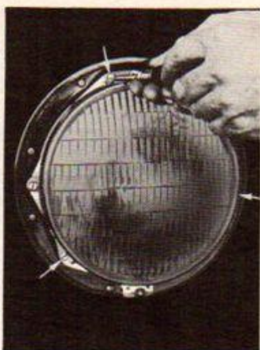
Fig. 38—Loosen Retaining Ring Screws
