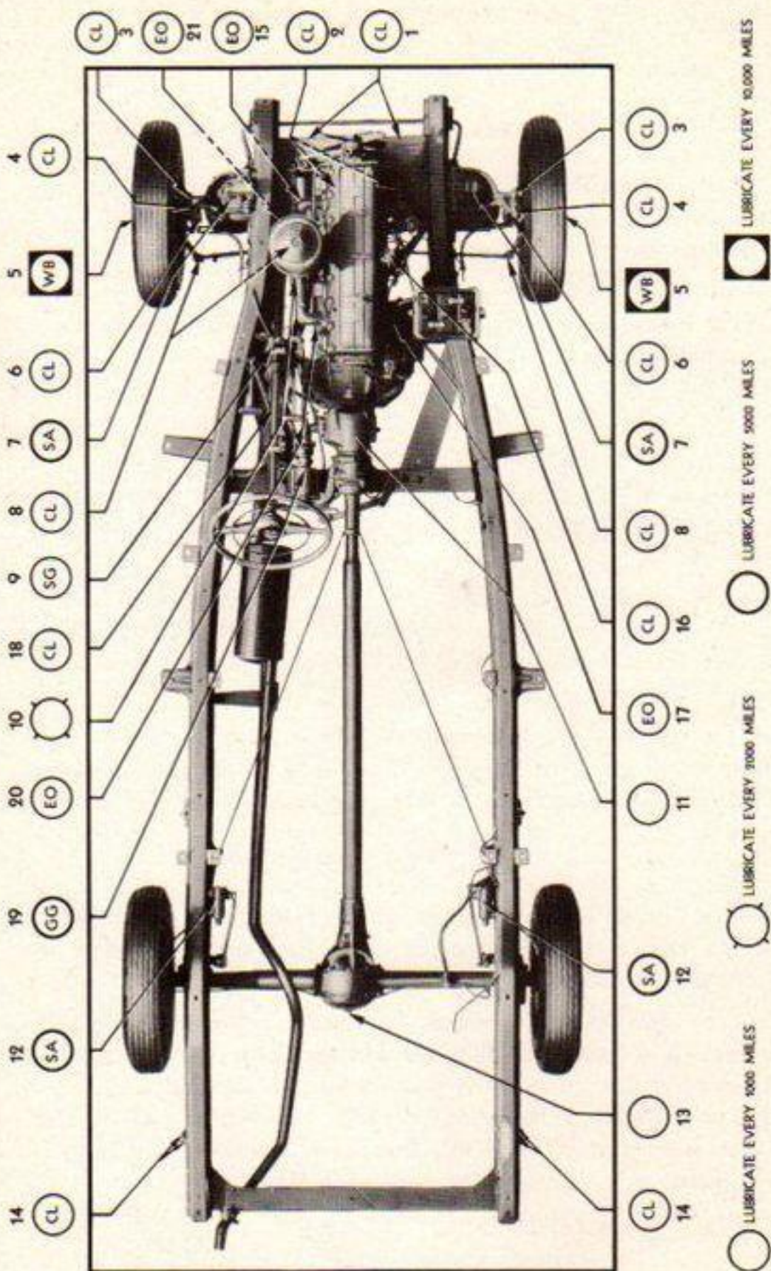
Fig. 43—Chassis Lubrication Chart
