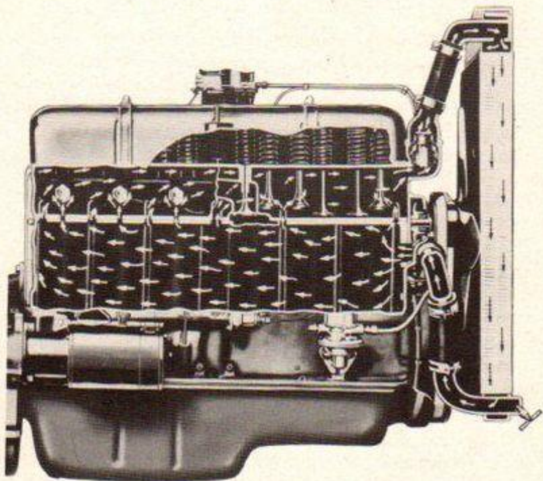
Fig. 30—Water Flow Through Engine
