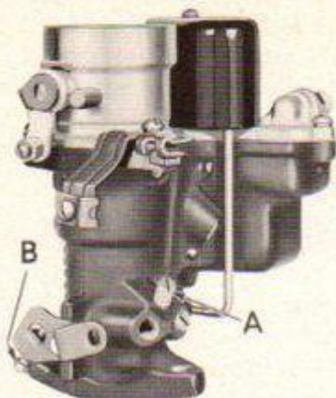
Fig. 27—Carburetor Adjustment
