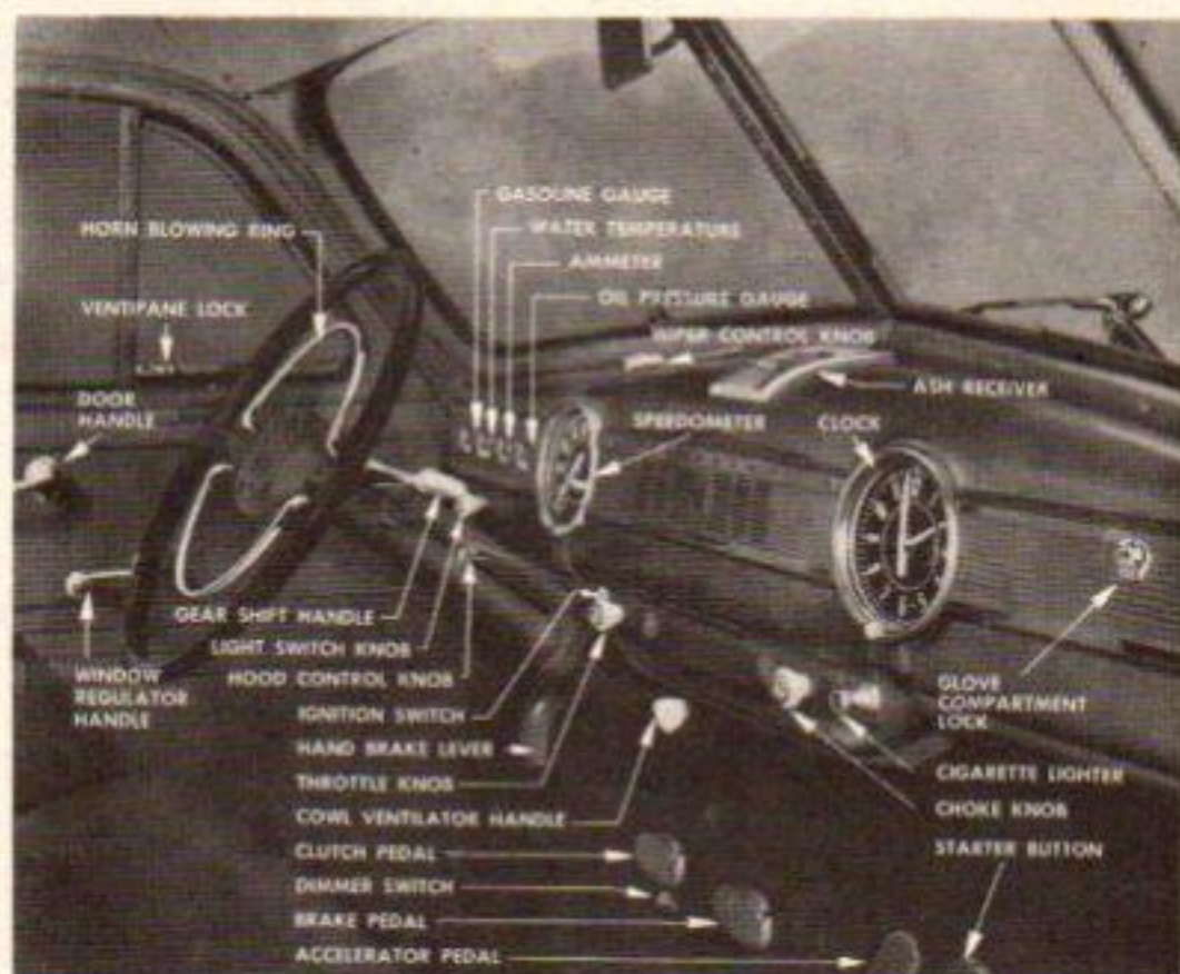
Fig. 1—Controls and Instruments—Fleetmaster and Fleetline
