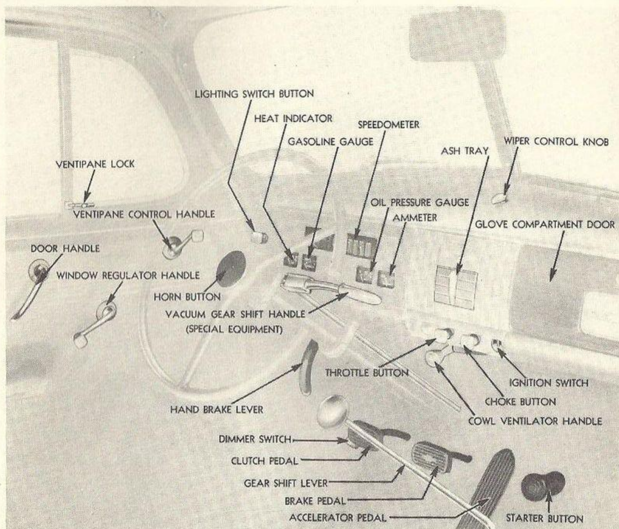
Fig. 1—Controls and Instruments (Master De Luxe Models)
