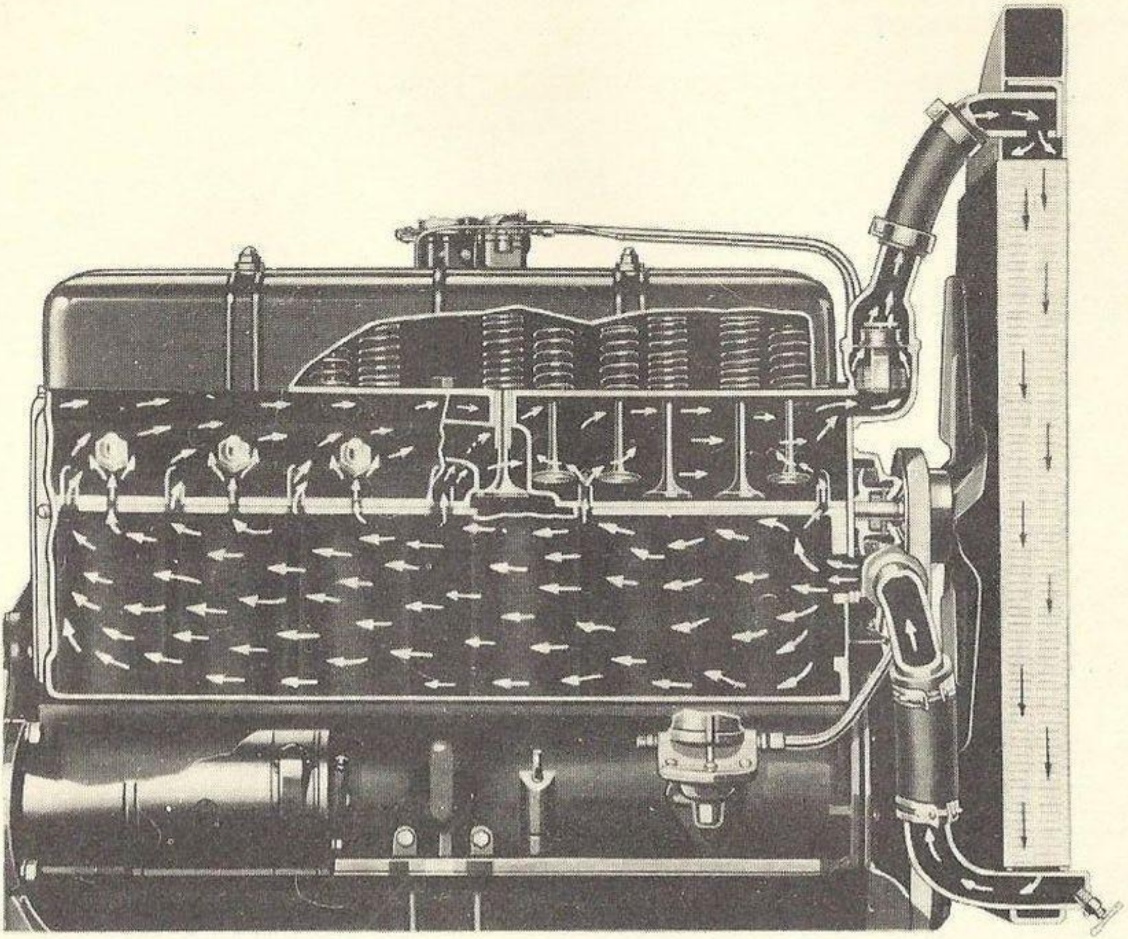
Fig. 32—Water Flow Through Engine
