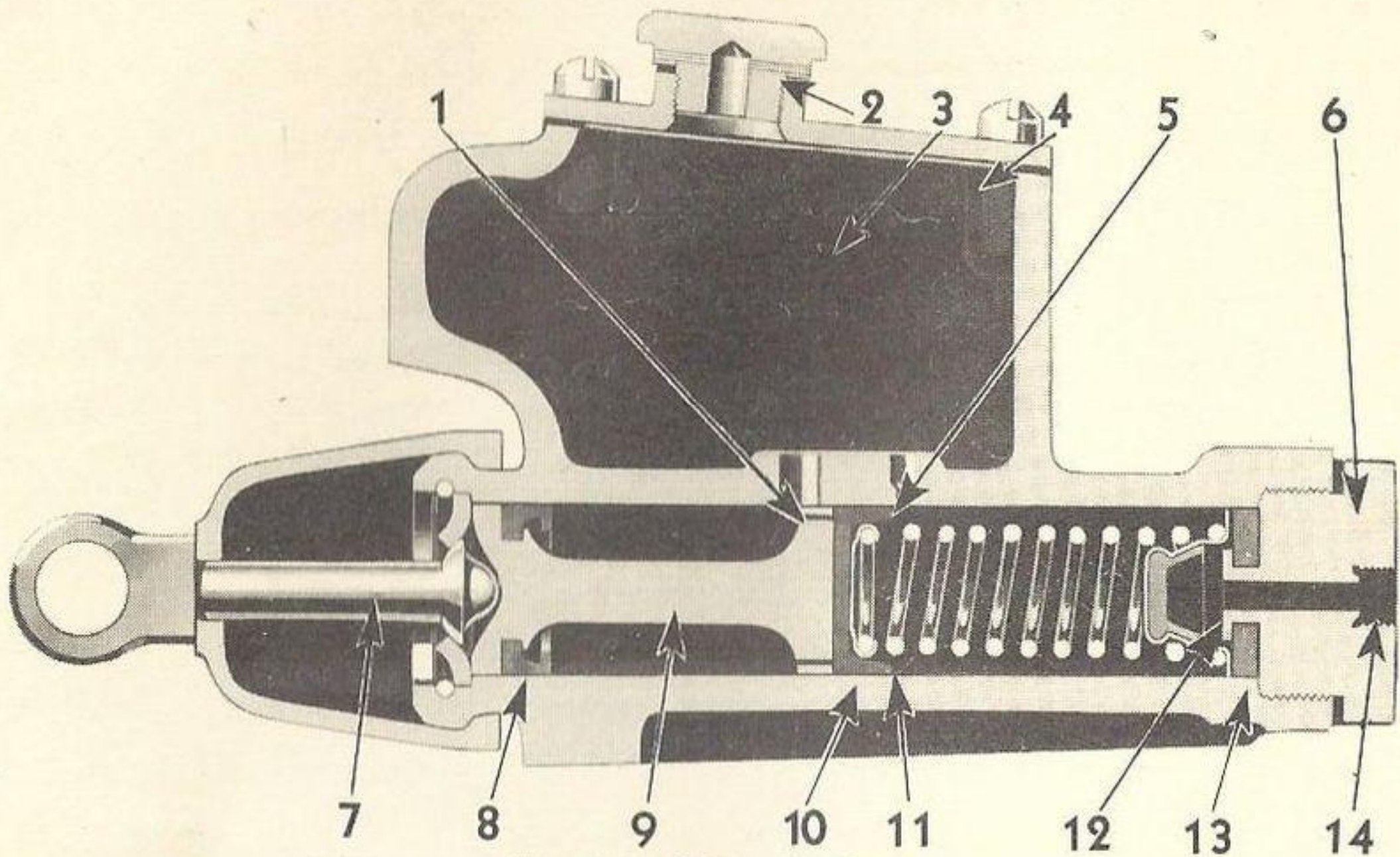
Fig. 26—Main Cylinder
