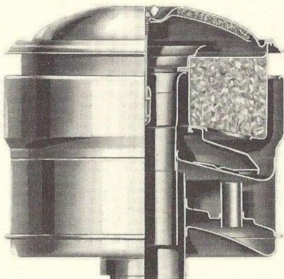
Fig. 31—Heavy Duty Air Cleaner
