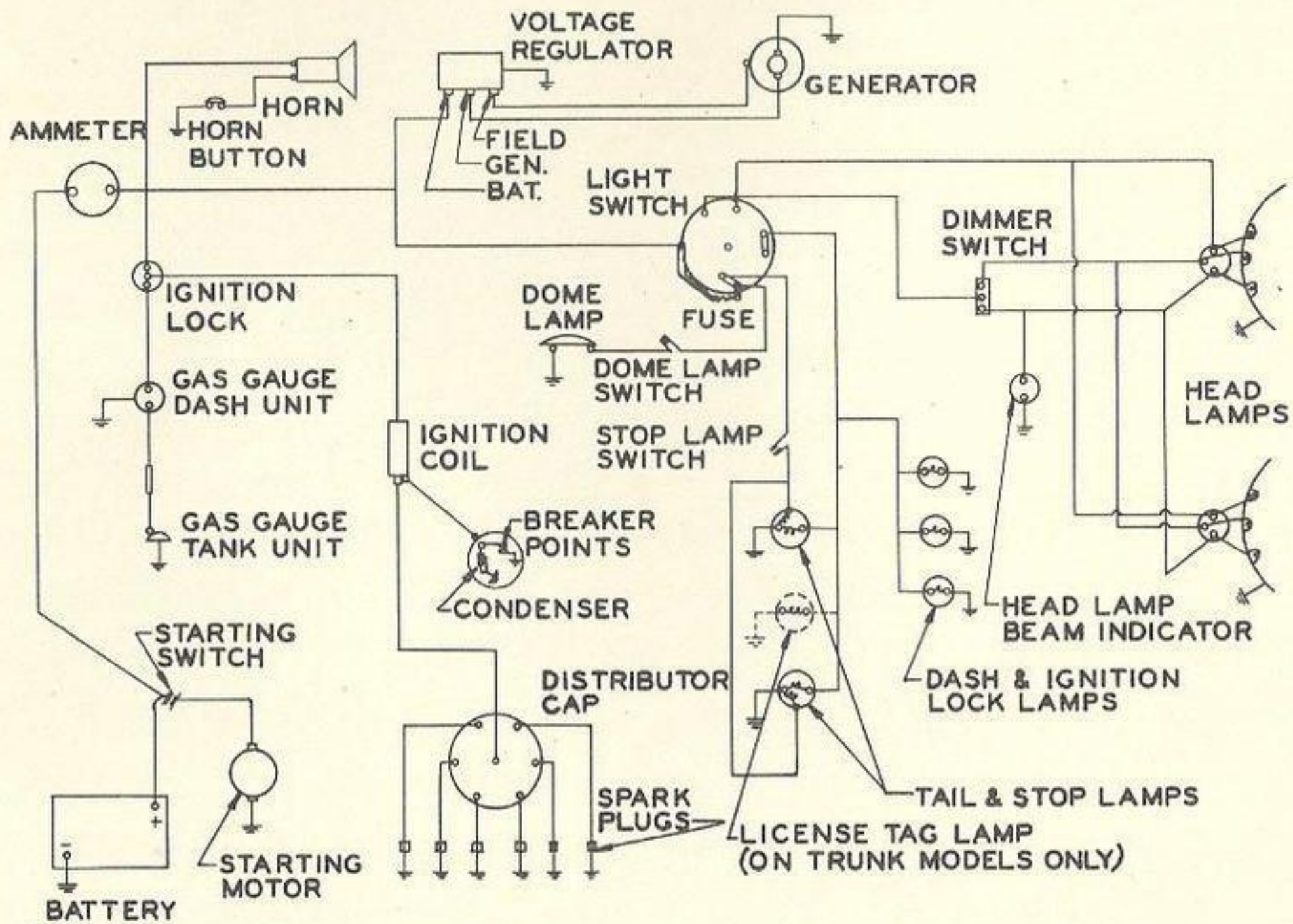
Fig. 33—Wiring Diagram
