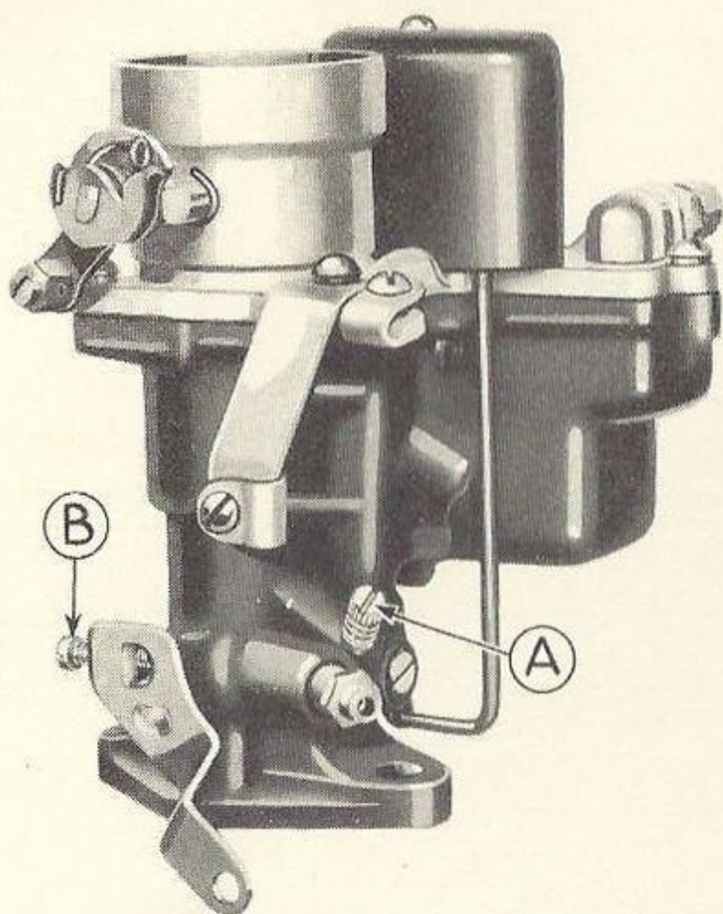
Fig. 28—Carburetor Adjustment
