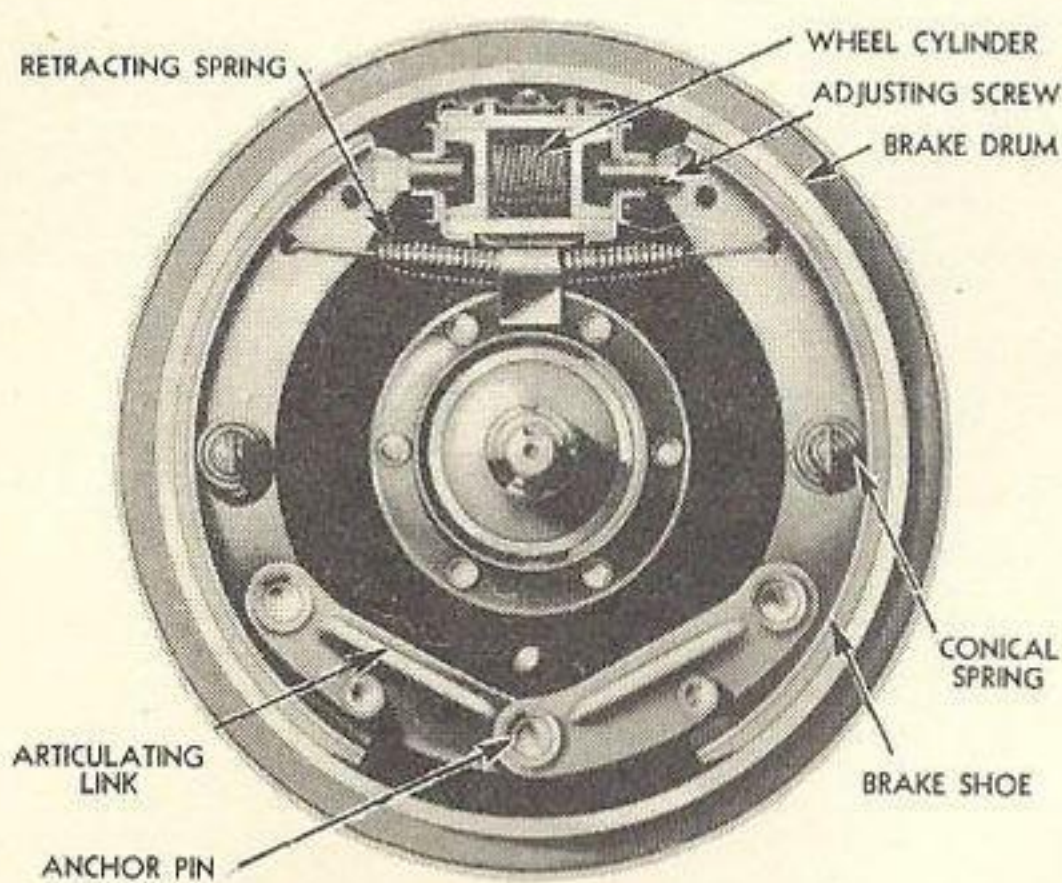
Fig. 27—Brake Mechanism at Front Wheel
