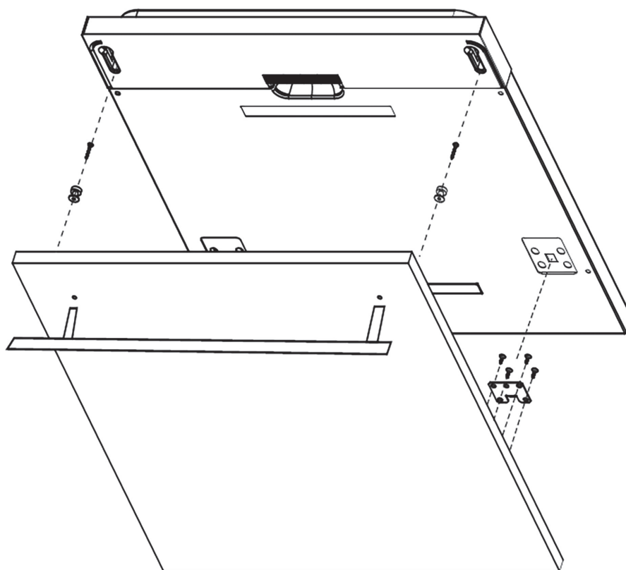
Figure 4a Installation of aesthetic panel
